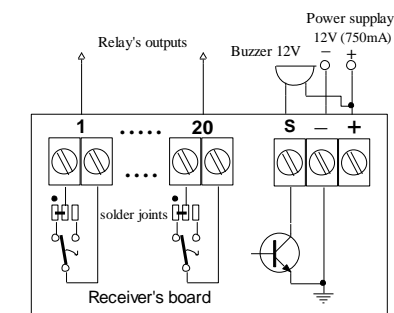
CH20H wiring diagram
